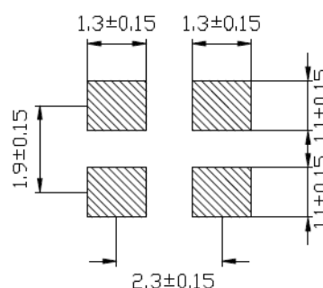
LAND PATTERN&lt;REFERENCE&gt;
