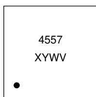
(DFN2x2-8L)
