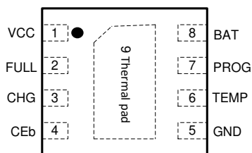
DFN2x2-8L(顶视图)
