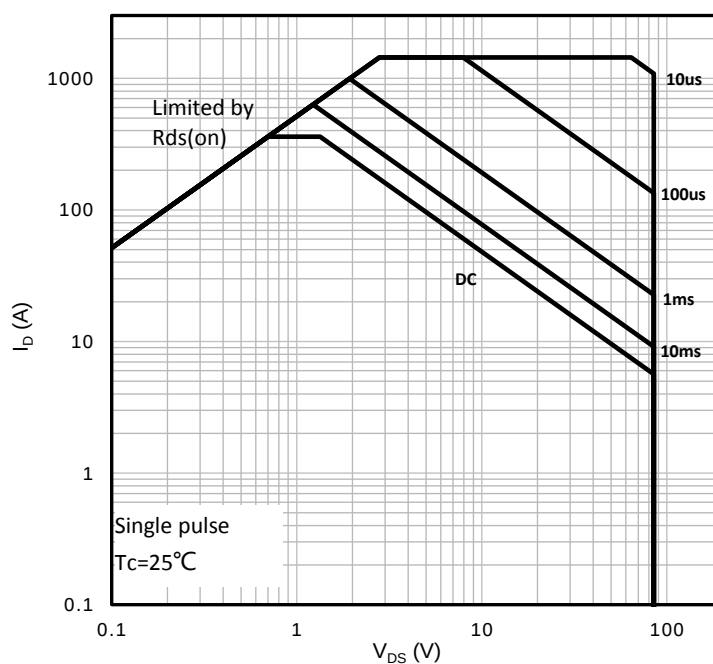
Figure 13. Safe Operating Area
