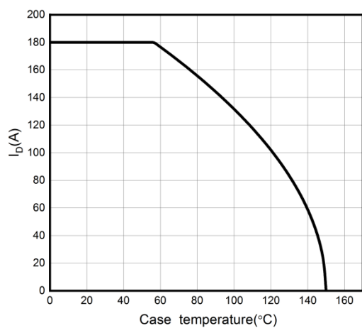
Figure 11. Drain Current Derating
