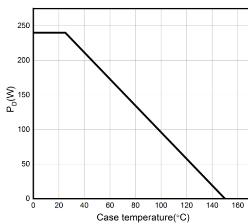
Figure 12. Power Dissipation vs. Temperature
