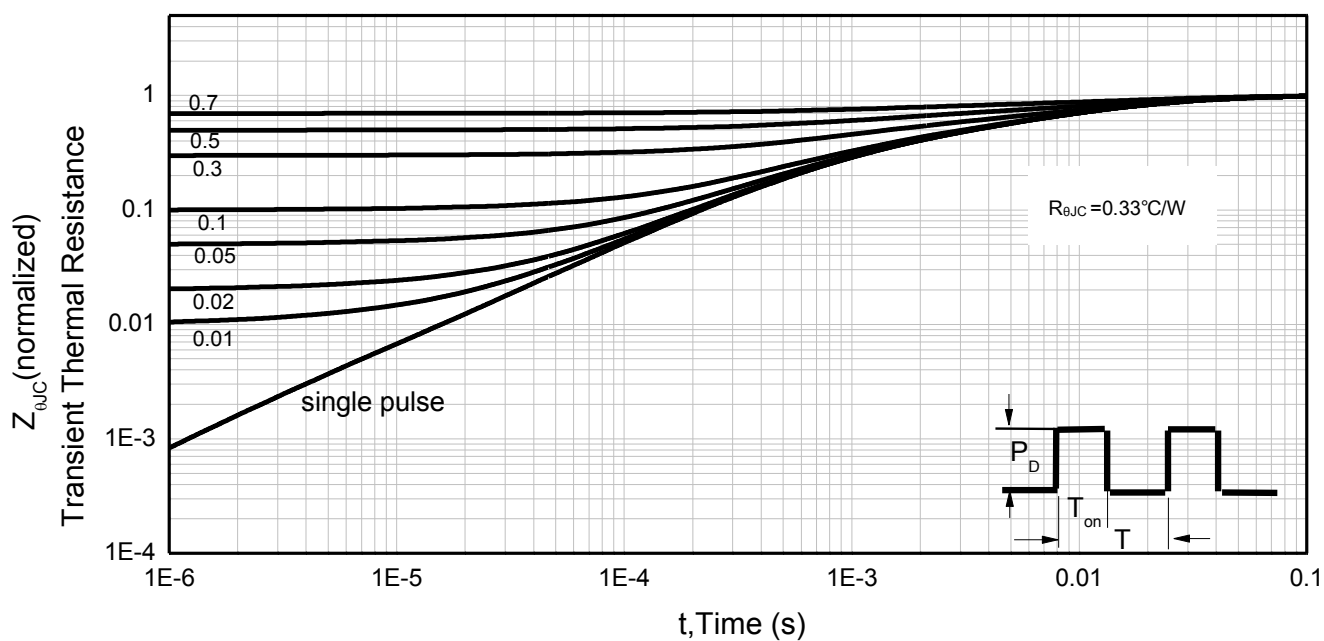
Figure 14. Normalized Maximum Transient Thermal Impedance ( R_{\theta JC} )
