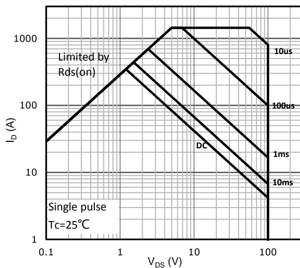
Figure 13. Safe Operating Area
