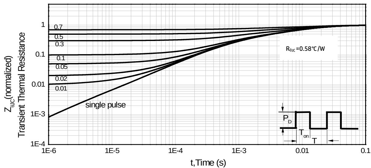
Figure 14. Normalized Maximum Transient Thermal Impedance ( R_{thJC} )
