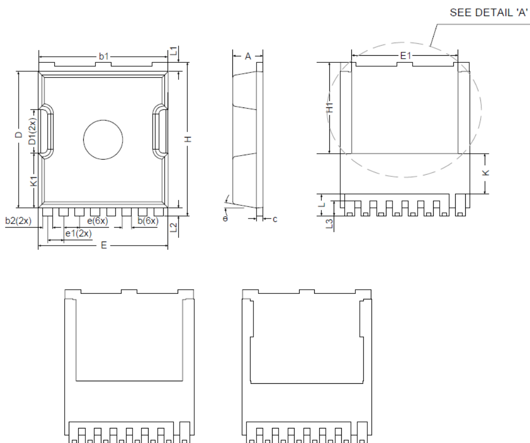
DETAIL 'A'
