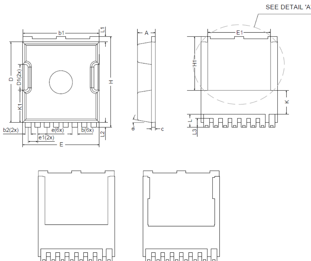
DETAIL 'A'
