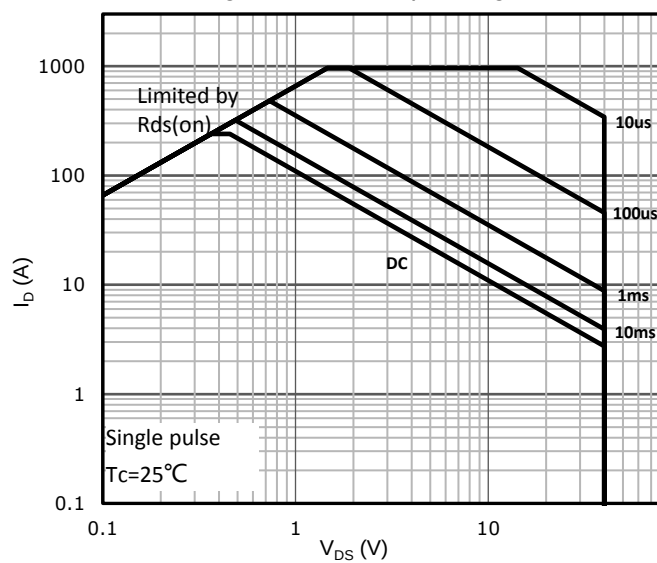
Figure 13. Safe Operating Area
