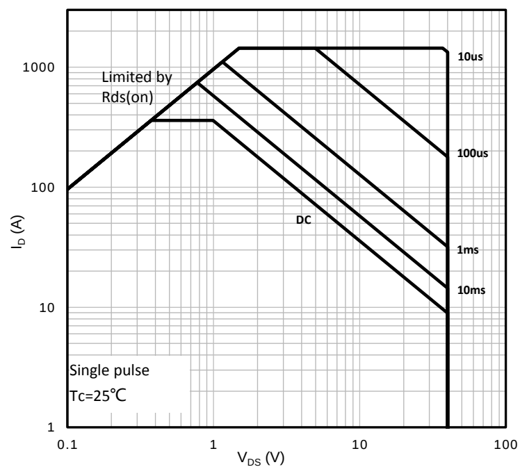
Figure 13. Safe Operating Area
