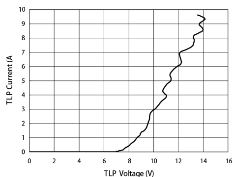
ESD Clamping of I/O_1 to I/O_2
