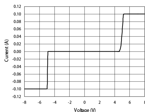
ESD Clamping of I/O_1 to I/O_2
